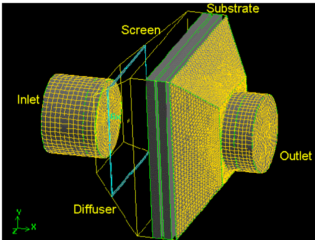
Fig. 5. The geometric configuration and part of the mesh.
